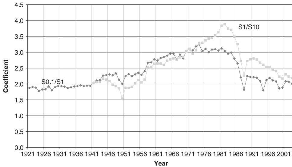
FIGURE 6 Pareto–Lorenz Coefficients
